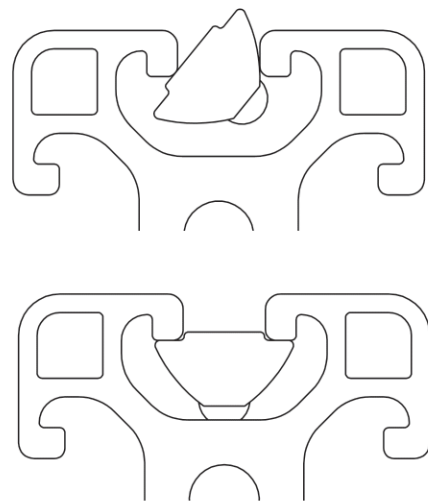
Positioning the T-slot nut
