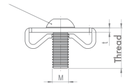
Screw, pan head, ISO 7380
