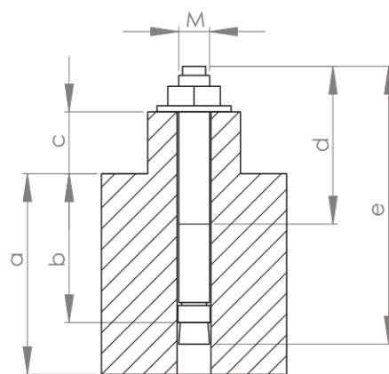
Floor dowel
